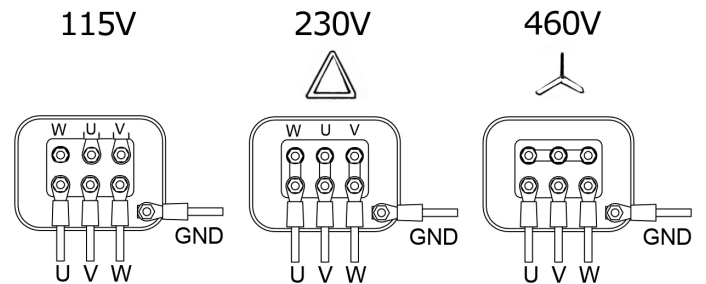
Fig. 4.4b MER terminal box wiring diagram
