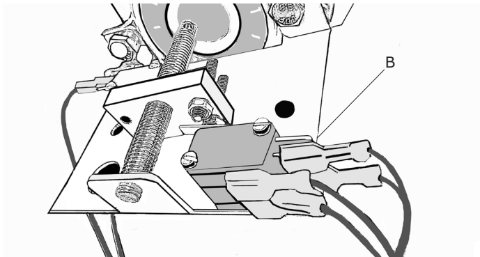
Fig. 1.4 MER hose limit switches with switch for controller.
