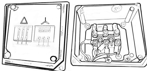
Fig. 4.4a Example of MER terminal box wiring
