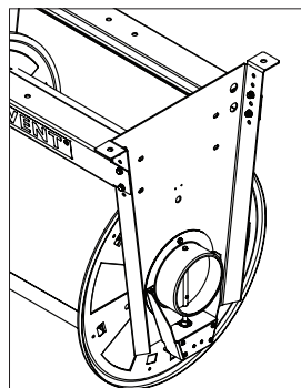
Fig. 4.5.3 Mechanical damper
