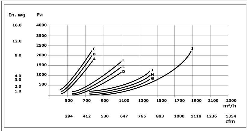
Fig. 5.1 Pressure loss by hose diameter and length
