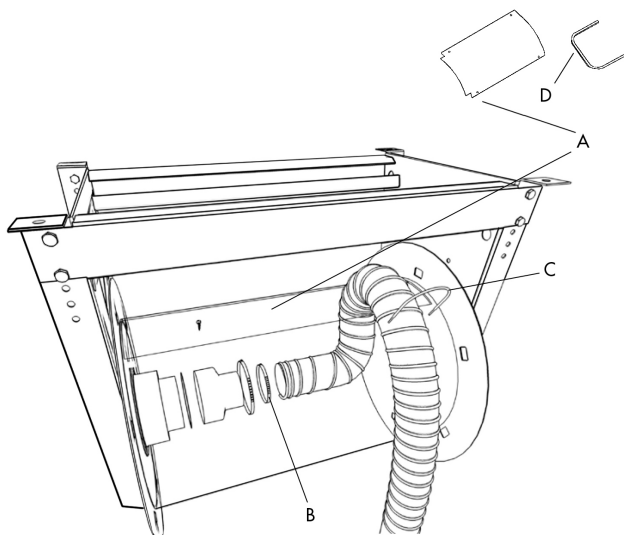
Fig. 4.1a Hose reel assembly
