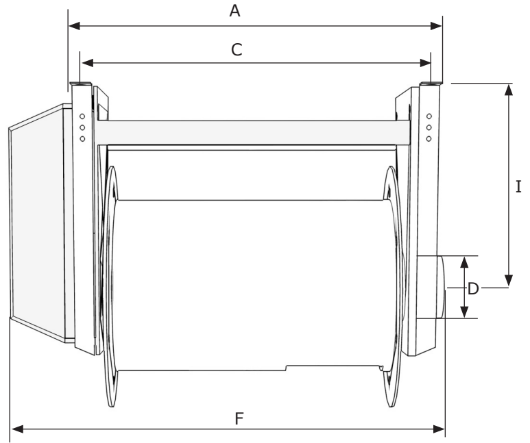
Fig. 4.2.2b Hose reel front view
