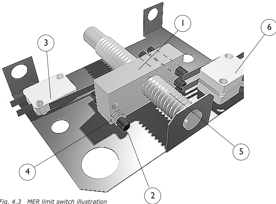
Fig. 4.3 MER limit switch illustration
