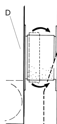
Fig. 4.5.1d Mounting the operating springs on the hose reel drum
