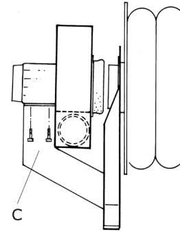
Fig. 4.5.1c Tightening the bolts on the DMF bracket
