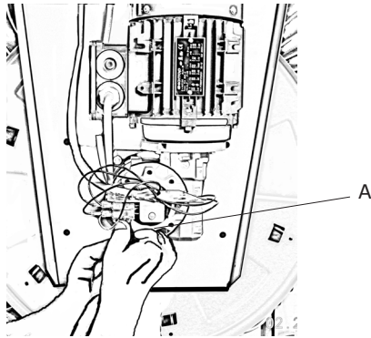
Fig. 1.3 Setting limit switches on MER
