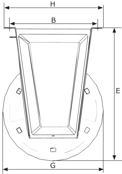
Fig. 4.2.2a Hose reel side view
