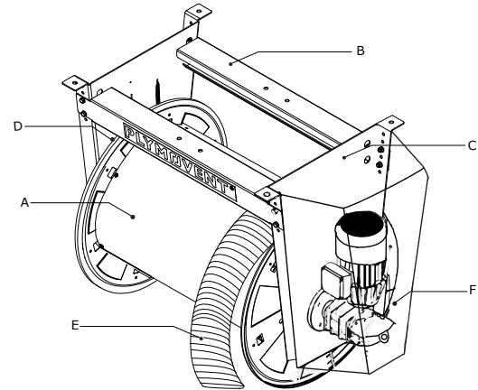
Fig. 1.1 MER hose reel with hose
