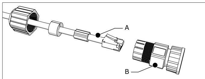
Fig. 4.19 Ethernet veld-connector
