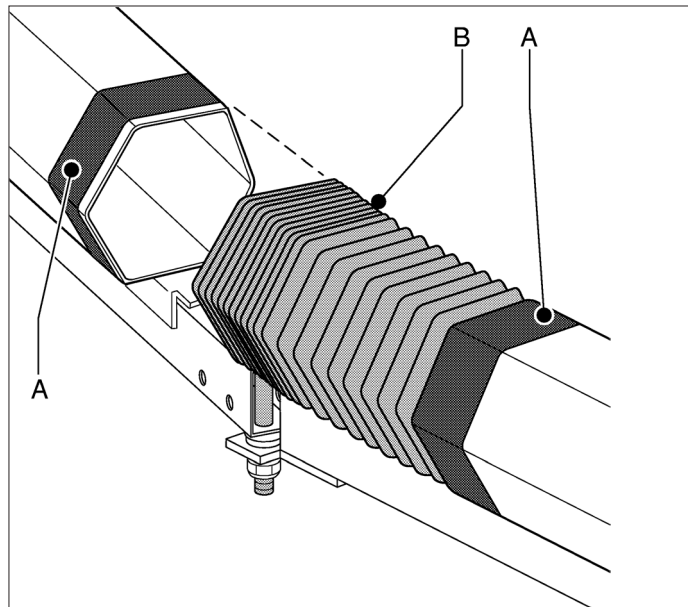
Fig. 4.4 Middle hose
