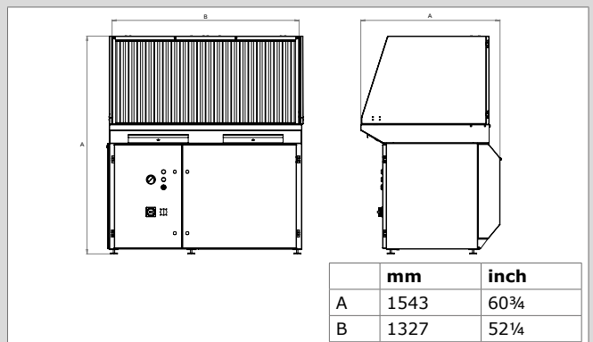
Downdraft table with backdraft kit and side panels (front view)
