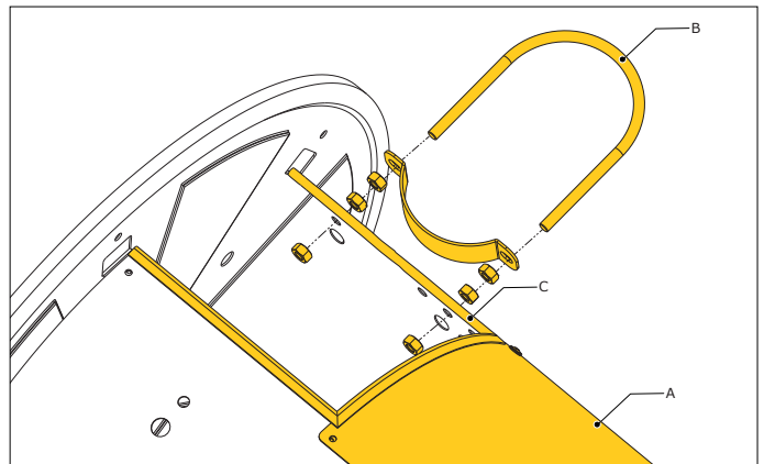
Fig. 6.10 Removing clamp, edge trim and drum
